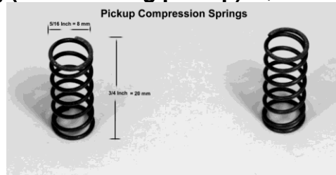
Two compression springs needed per pickup.
