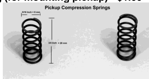
#PU-069 – Compression Spring (for mounting pickup) - $1.00
